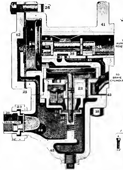
Fig. 1751. Quick-action Triple-valve.
